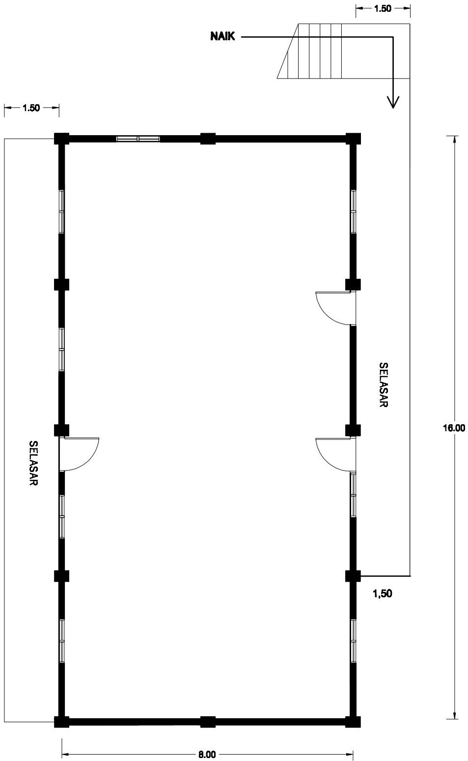
DENAH LT.2 - GEDUNG F Scale 1:100
