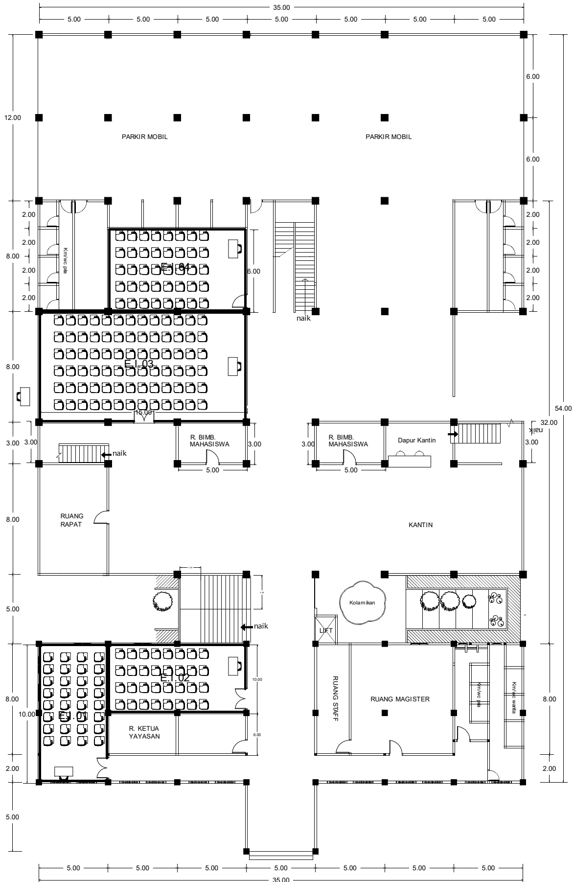
DENAH LANTAI 1
